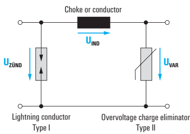
This used to be the usual solution, because the arresters were not co-ordinated.
